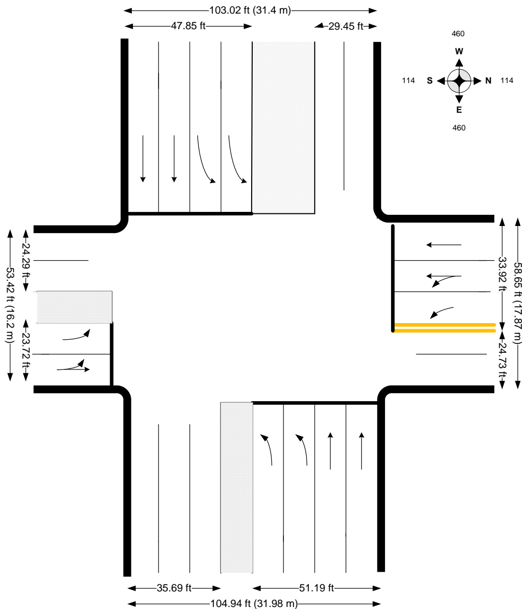
Figure 7. Illustration. Diagram of Peppers Ferry (VA-114) & Franklin (Bus460) intersection.
