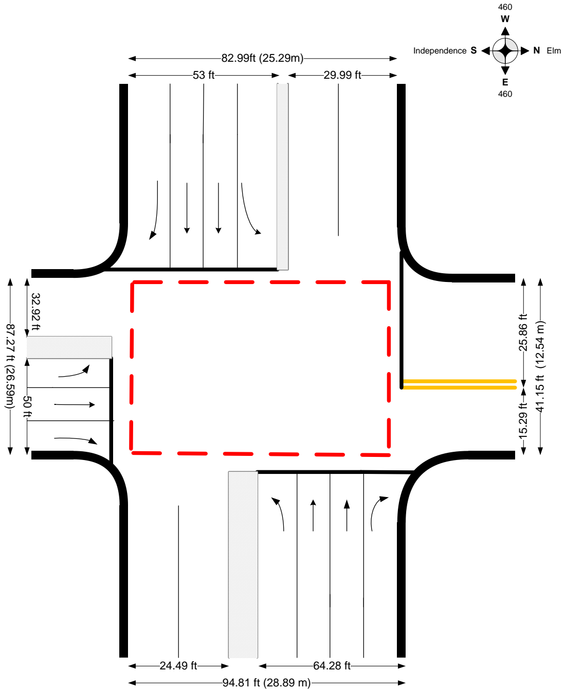
Figure 1. Illustration. Diagram of Franklin, Elm & Independence intersection.
