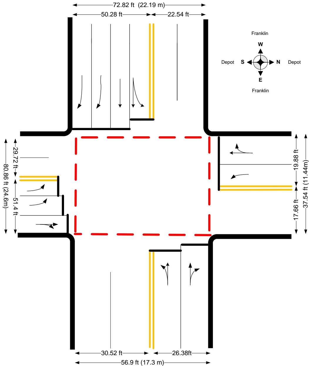
Figure 4. Illustration. Diagram of Depot & Franklin intersection.
