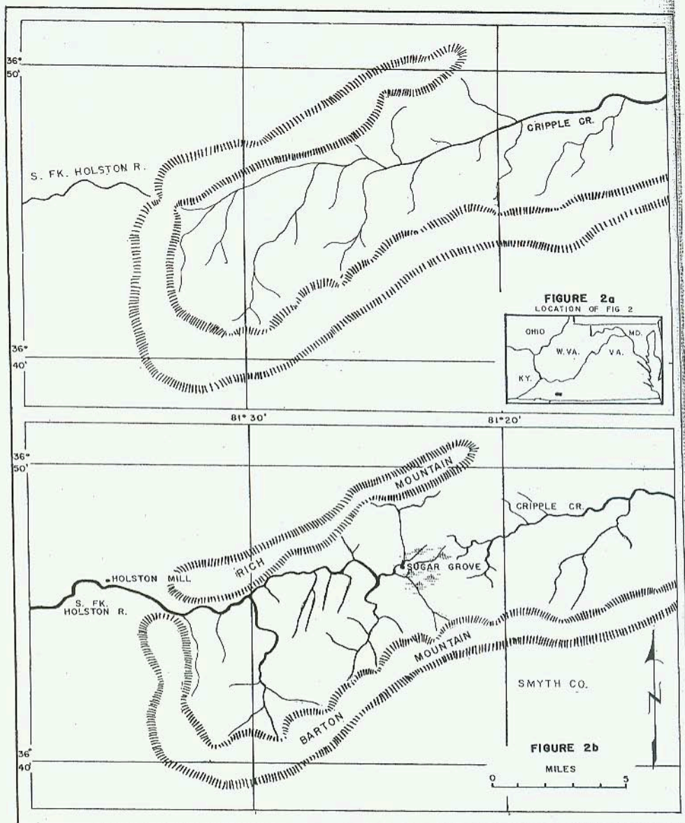
Fig. 2. Stream capture at Sugar Grove, Smyth County, Virginia. Fig. 2a: Prior to capture, drainage to Cripple Creek of New River. Fig. 2b: Present drainage to South Fork of Holston River after beheading of upper Cripple Creek.
