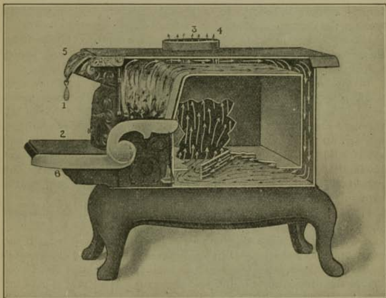
FIG. 18.—A modern coal range.
