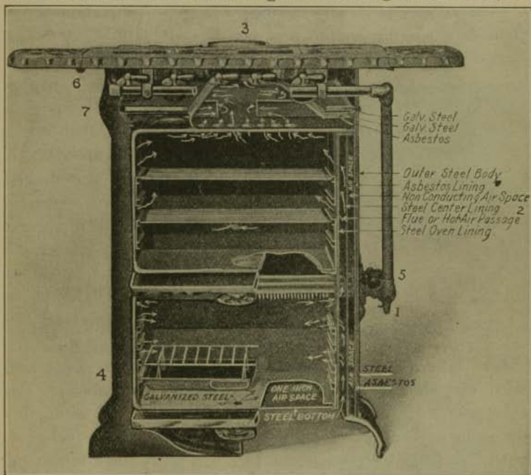
FIG. 19. — A modern gas range.
