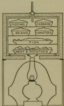
FIG. 16.—The Atkinson cooker.
