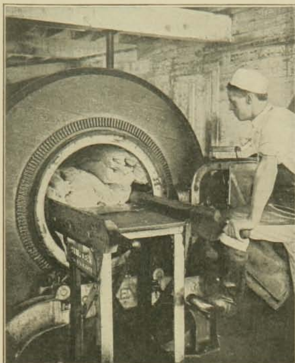
A modern churn which first converts the ripened cream into butter and then thoroughly works and salts it
