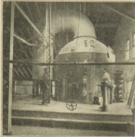
Vacuum Pan for final Crystallizing
