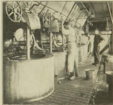
Centrifugal machines, to separate the syrup from the sugar crystals
